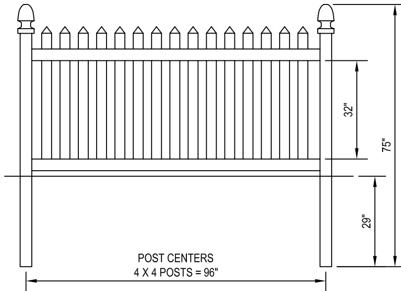
DANBURY, THRU PICKET STYLE 4' HIGH / 8' WIDE
