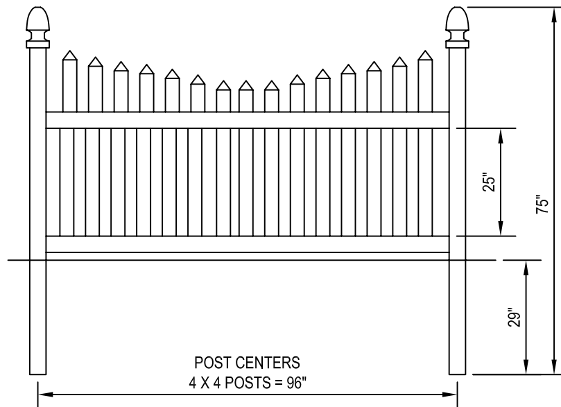
DANBURY CONCAVE, THRU PICKET STYLE 4' HIGH / 8' WIDE
