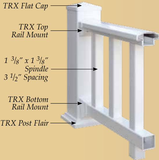
TRX Rail Aluminum Reinforcement
